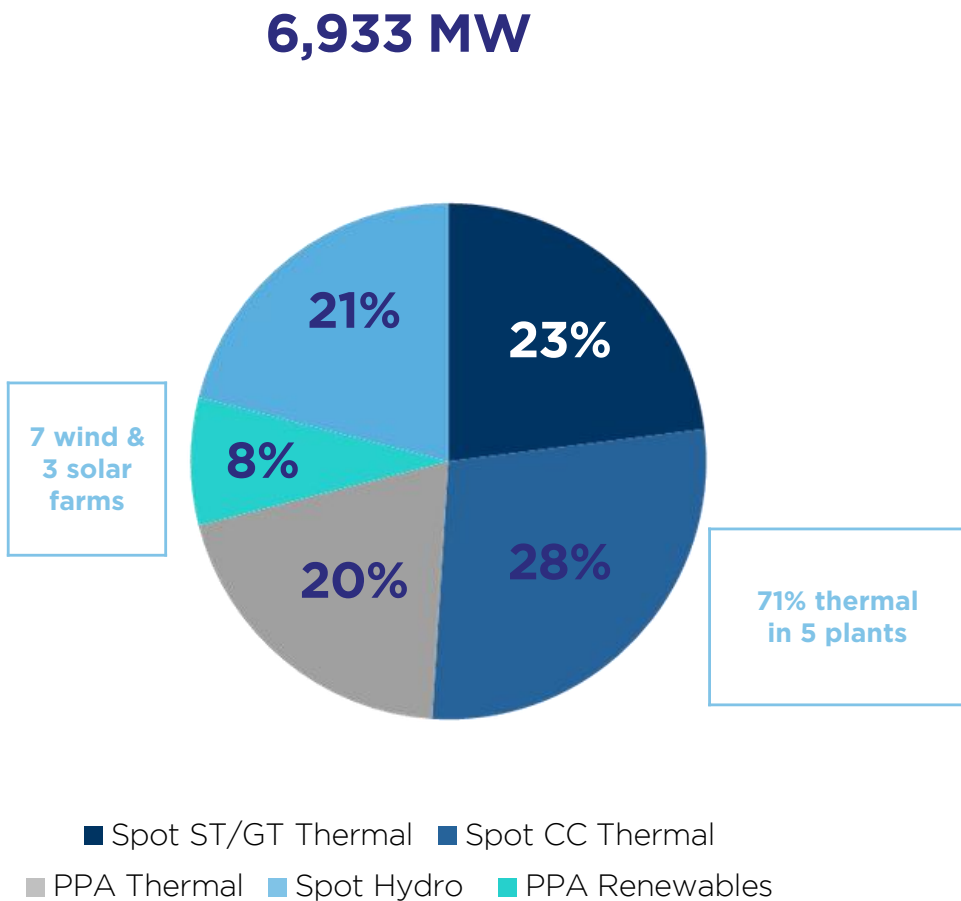
2025 Installed capacity breakdown by technology mix and revenue model:
